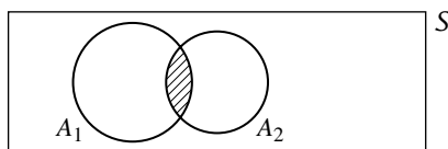
Figure 1.4 A_1 \cap A_2 is the shaded region.
